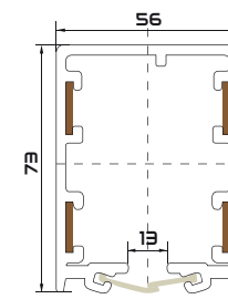
4P:35A-100A(IP43)
